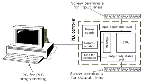
Figure 4: Basic elements of PLC controller [1]
