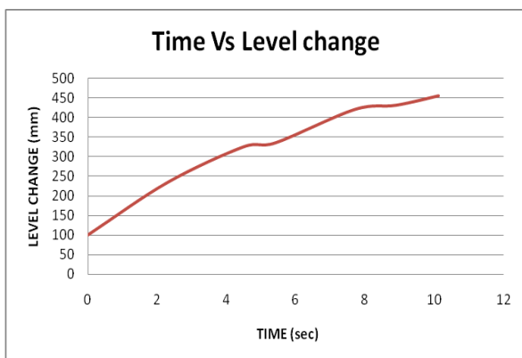
Figure 17: Time versus water level change of PID Controller.
