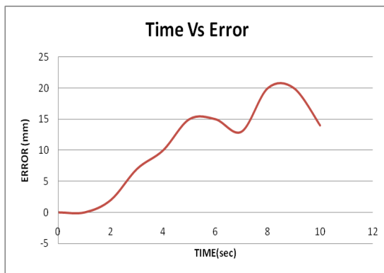
Figure 22: Time versus error of PLC.
